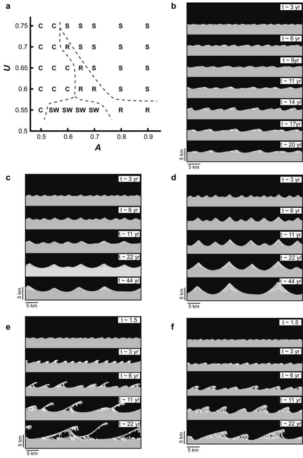
Figure 9. (a) Different modes of simulated shoreline response as U and A are varied. C represents cuspsate bumps, SW represents alongshore sand waves, R represents reconnecting spits, and S indicates flying spits. Also shown are progressive stacks of the plan view model domain demonstrating typical simulation responses: (b) migrating alongshore sand waves (SW, A = 0.65, U = 0.55 ), (c) subtle cuspsate bumps (C, A = 0.5, U = 0.6 ), (d) more pronounced cuspsate bumps (C, A = 0.5, U = 0.7 ), (e) flying spits (S, A = 0.7, U = 0.65 ), and (f) reconnecting spits (R, A = 0.7, U = 0.6 ). Cells along the shoreline are plotted with a shading brightness proportional to the fractional amount of sediment within the cell. Sediment deposited contemporaneously is plotted with the same color. Animations of these simulations can be in the auxiliary material.
