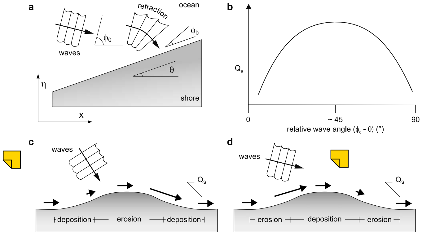
Figure 1. Illustrations depicting the high wave angle instability in shoreline shape. (a) Depiction of terms and axes. (b) Schematic of the relationship between alongshore sediment transport ( Q_s ) and relative wave angle ( \phi_0 - \theta ), showing a maximum in Q_s for (\phi_0 - \theta) \approx 45^\circ . (c) Response of a perturbation to a plan view shoreline subjected to low-angle waves ( (\phi_0 - \theta) < \sim 45^\circ ). Sediment flux increases down-drift along the flanks and increases along the crest, resulting in flattening of the shape. (d) Opposite response for high-angle waves, with erosion along the flanks where (\phi_0 - \theta) is decreasing ( Q_s diverging) and accretion along the crest as (\phi_0 - \theta) increases ( Q_s converging).
