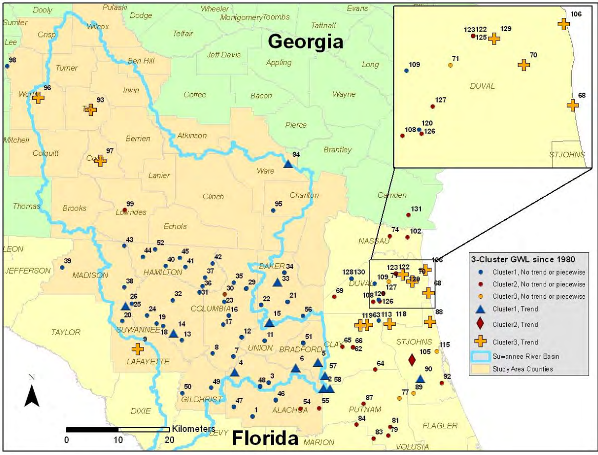
Figure 9.3. 3-Cluster Plot and Map. (A) Averages of normalized groundwater levels for clusters 1 (blue), 2 (red), and 3 (yellow). (B) Spatial distribution of the groundwater wells for clusters 1 (blue), 2 (red), and 3 (yellow).
