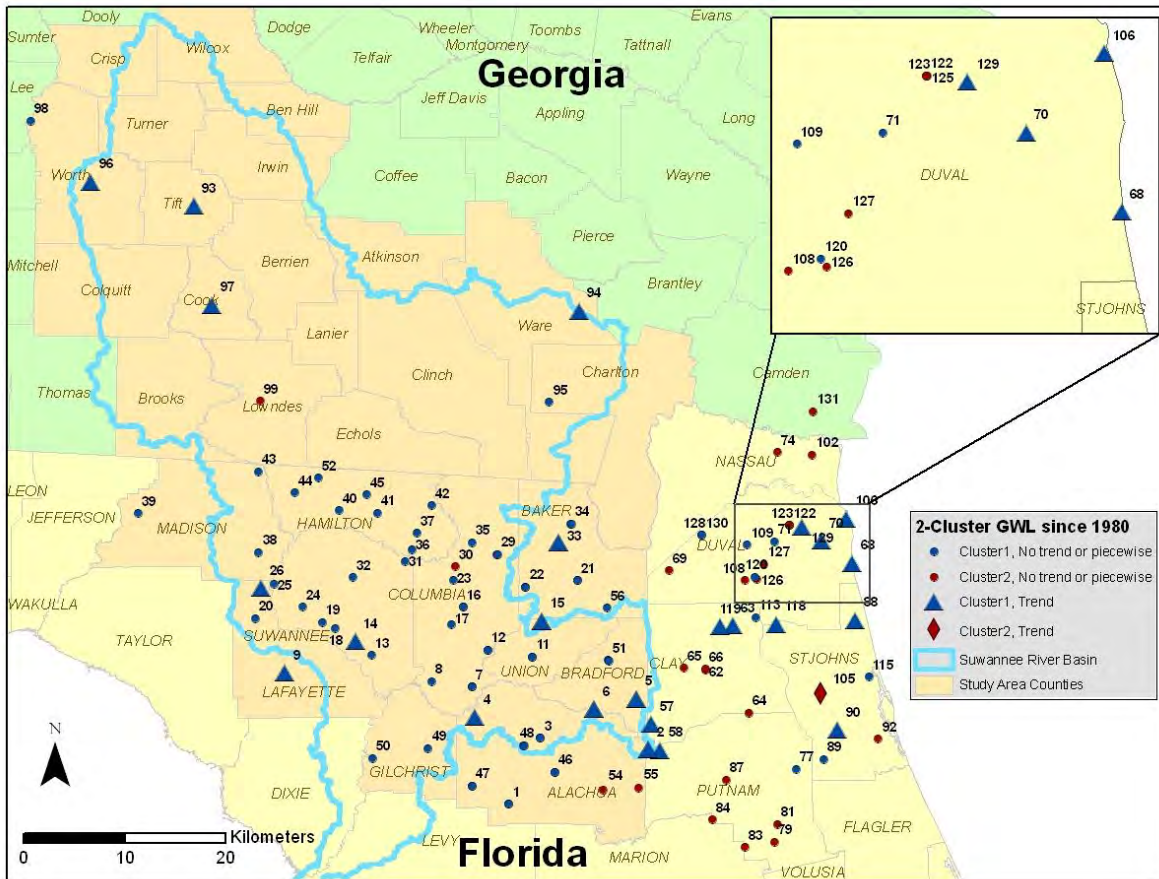
Figure 9.2. 2-Cluster Plot and Map. (A) Averages of normalized groundwater levels for clusters 1 (blue) and 2 (red). (B) Spatial distribution of the groundwater wells for clusters 1 (blue) and 2 (red).
